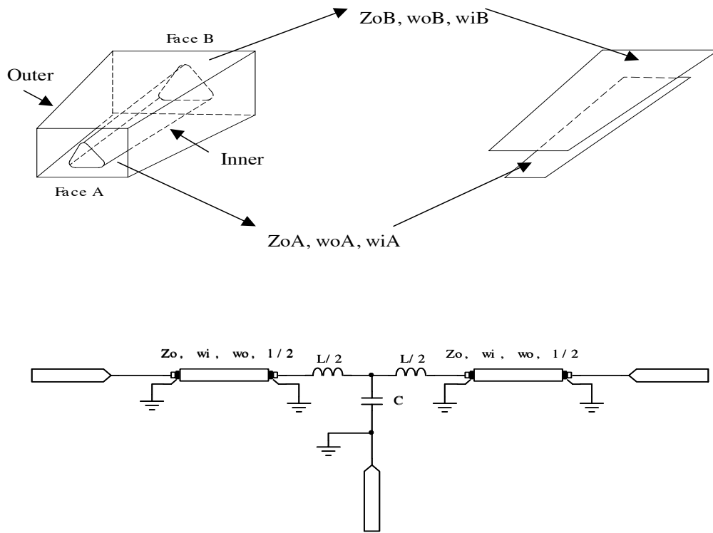
Figure 1: An illustration of the process of converting a mechanical segment of transmission line to its equivalent circuit representation.
