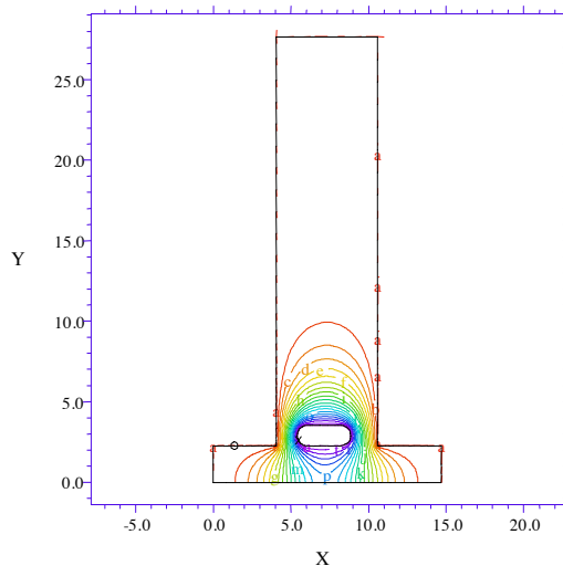
Figure 2: An example numerical analysis performed on a typical K250 cyclotron cross-section.
