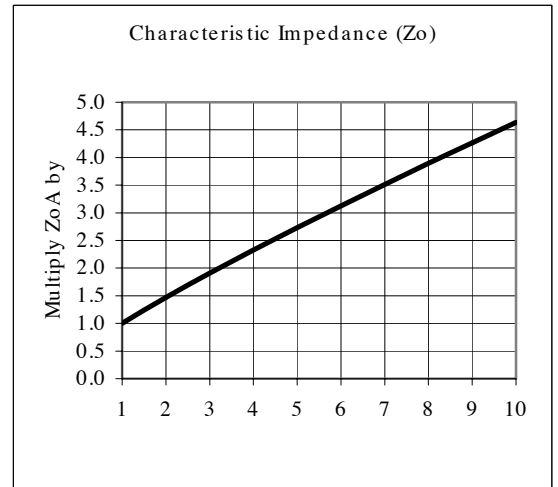
Figure 3: Graphs used to determine the values for the elements of the equivalent circuit in lieu of applying the formula.
